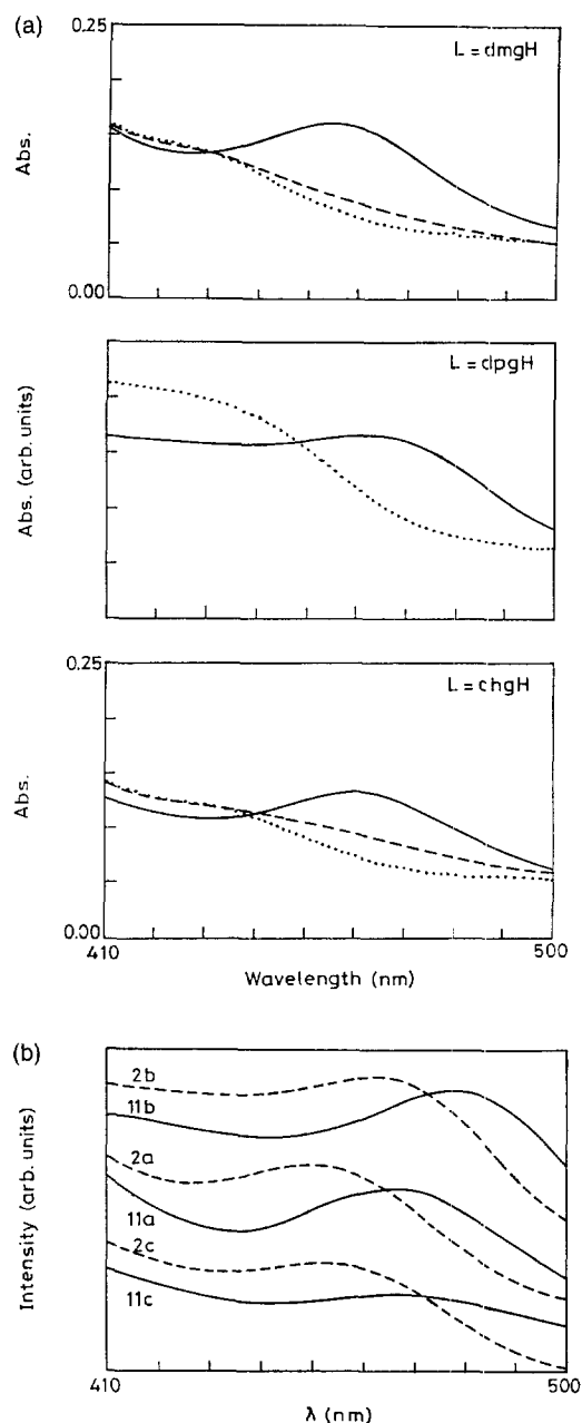
Fig. 2. (a) Effect of the addition of pyridine (— 0.0 M, --- 10^{-3} M, \cdots 10^{-2} M saturation curve) to a 10^{-5} M solution of n\text{Bu}(\text{L}_2)\text{Py} in methanol ( \text{L} = \text{dmgH} , \text{chgH} ). 4a , 4b for \text{L} = \text{dpgh} ; 4c , the plot is qualitative (see text). (b) Appearance of Co–C CT band of 2 and 11(a,b,c) in methanol.
