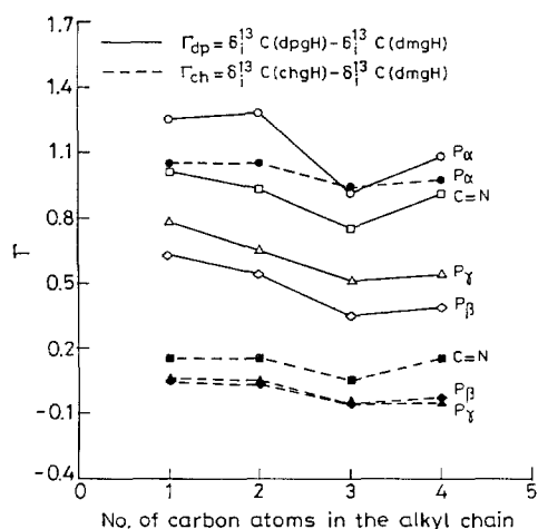
Fig. 5. Variation of Cis influence ( F ) on the carbon atoms of the \{Co(L)_2\} moiety with increasing alkyl chain length.
