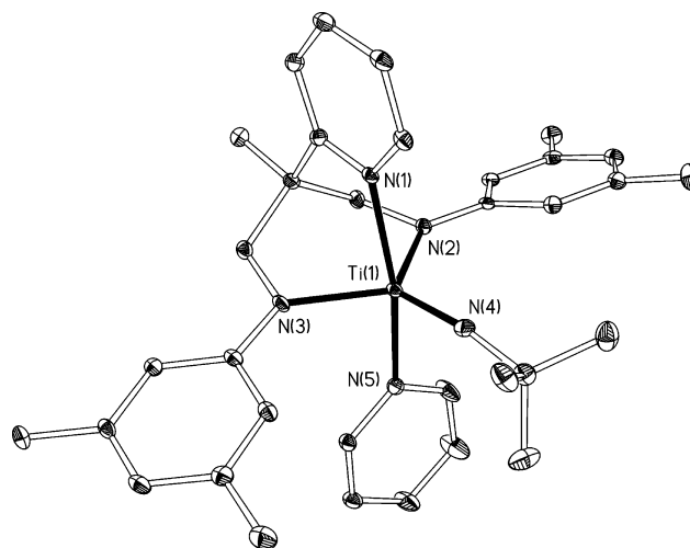
Figure 2. Molecular structure of [\text{Ti}(\text{N}^i\text{Bu})(\text{N}_2^{\text{XylNpy}})(\text{py})] 3c . Ellipsoids are drawn at the 25% probability level and H atoms are omitted for clarity. Selected bond lengths (Å) and angles (deg): Ti(1)–N(1) 2.202(2), Ti(1)–N(2) 1.985(2), Ti(1)–N(3) 2.018(2), Ti(1)–N(4) 1.706(3), Ti(1)–N(5) 2.241(2), N(1)–Ti(1)–N(2) 80.37(9), N(1)–Ti(1)–N(3) 81.83(10), N(2)–Ti(1)–N(3) 116.64(10), N(1)–Ti(1)–N(4) 102.82(10), N(2)–Ti(1)–N(4) 119.85(11), N(3)–Ti(1)–N(4) 123.31(11), N(1)–Ti(1)–N(5) 163.22(9), N(2)–Ti(1)–N(5) 89.94(10), N(3)–Ti(1)–N(5) 90.48(10), N(4)–Ti(1)–N(5) 93.87(10), Ti(1)–N(4)–C(26) 170.5(2).
