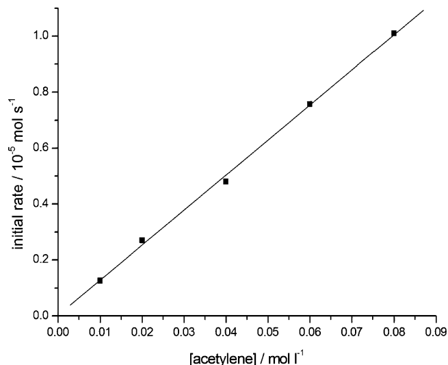
Figure 6. Plot of the initial rate versus concentration of alkyne for the reaction of 10 μmol of [\text{Ti}(\text{N}'\text{Bu})(\text{N}_2^{\text{Xyl}}\text{N}_{\text{py}})(\text{py})] 3c with varying amounts of phenyl acetylene.
