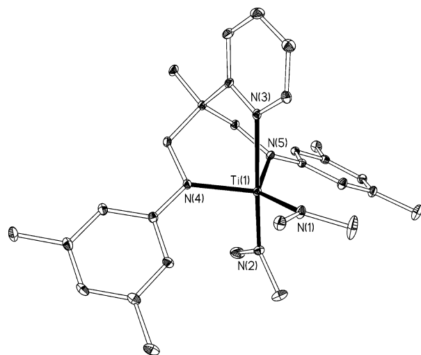
Figure 1. Molecular structure of [\text{Ti}(\text{N}_2^{\text{XylNpy}})(\text{NMe}_2)_2] 2b . Ellipsoids are drawn at 25% probability, and H atoms are omitted for clarity.
