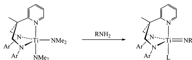
Scheme 2. Synthesis of the Imido Complexes 3a – 3e
