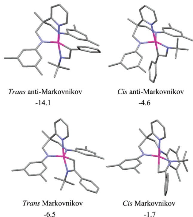
Figure 5. ONIOM calculated structures for the isomeric forms of [\text{Ti}(\text{N}_2^{\text{Xyl}}\text{N}_{\text{py}})\{\kappa^2\text{-N}(\text{'Bu})\text{CHC}(\text{Ph})\}] 4c . Energies are provided in kcal mol -1 .
