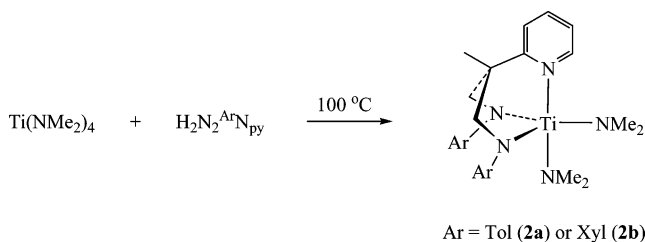
Scheme 1. Synthesis of [\text{Ti}(\text{N}_2^{\text{Ar}}\text{Npy})(\text{NMe}_2)_2] 2a and 2b
