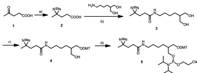
Fig. 1 Synthesis of diazirine phosphoramidite: (a) 1 \text{NH}_3 (liquid), \text{NH}_2\text{O-SO}_3\text{H} , MeOH; 2 \text{I}_2 , \text{Et}_3\text{N} , MeOH, 0 °C; (b) DCC, HOBT, DMF, room temperature, 24 h; (c) DMT-Cl, pyridine, \text{CH}_2\text{Cl}_2 , DMAP, ice bath, and then room temperature about 24 h; (d) \text{P-(N-iPr}_2)_2(\text{OCH}_2\text{CH}_2\text{CN}) , DIPEA, \text{CH}_2\text{Cl}_2 , 0 °C, about 4 h.
