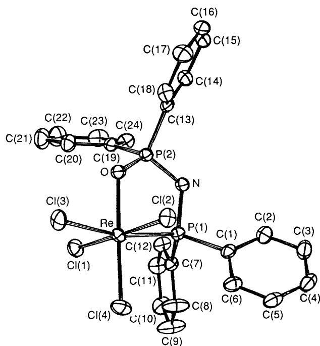
Fig. 4 An ORTEP view of the anion complex 4 showing the thermal ellipsoids at 30% probability
