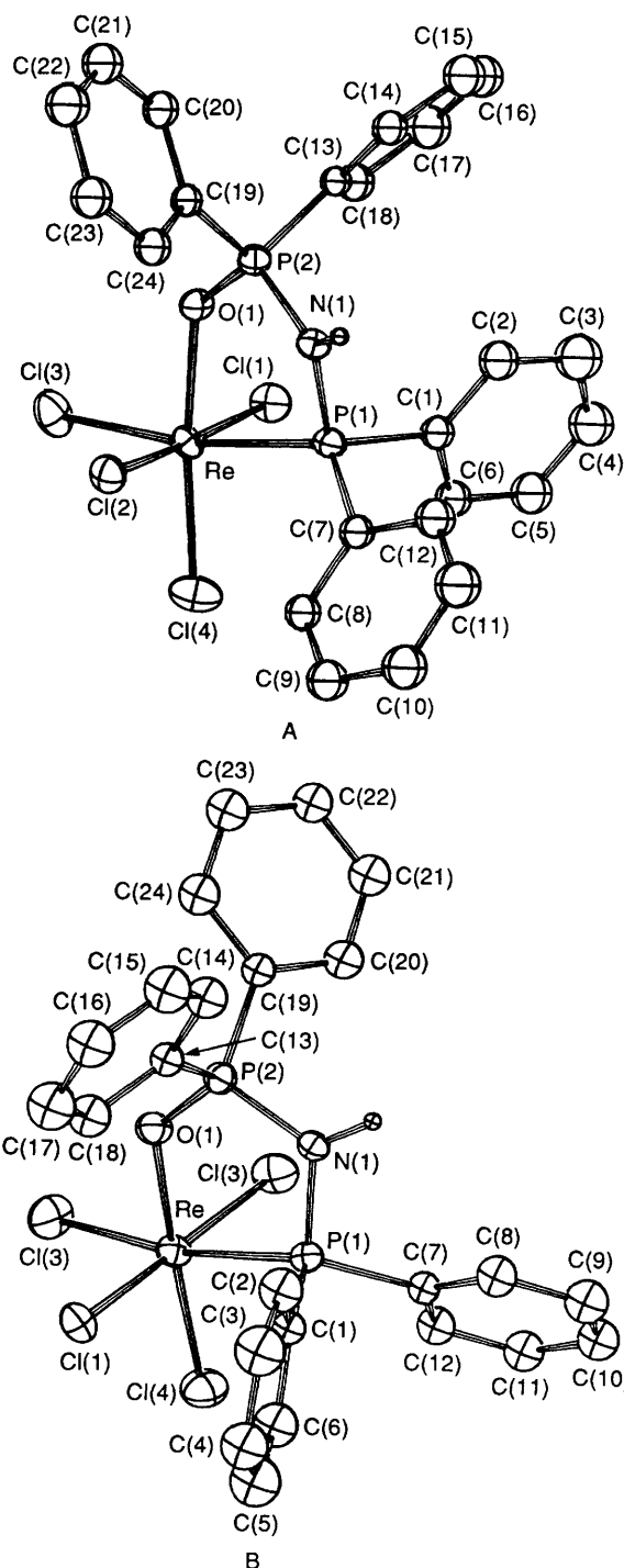
Fig. 2 The ORTEP views of the two independent molecules A and B of complex 3 showing the thermal ellipsoids at 30% probability
