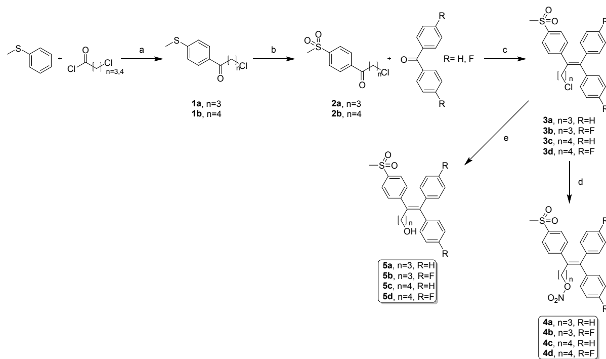
Fig. 2: Synthetic pathway of NO-releasing SERMs (4) and reference SERMs (5). Reagents and conditions: (a) \text{AlCl}_3 , \text{CHCl}_3 , argon, 2.5 h rt, (b) oxone® (potassium peroxymonosulphate), \text{MeOH/THF} (1/1, v/v), 31 h, (c) \text{Zn} , \text{TiCl}_4 , reflux 4.5 h, (d) \text{AgNO}_3 , \text{MeCN} , 24 h, 80^\circ\text{C} , (e) \text{CuSO}_4 \times 5 \text{ H}_2\text{O} , \text{DMSO/H}_2\text{O} (1/3, v/v), 130^\circ\text{C} , 48 h.
