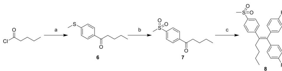
Fig. 3: Synthetic pathway of SERM 8. Reagents and conditions: (a) thioanisole, \text{AlCl}_3 , \text{CHCl}_3 , 1.5 h, rt (b), oxone® (potassium peroxydisulfate), MeOH/THF (1/1, v/v), 15 h, (c) 4,4'-difluorobenzophenone, Zn, \text{TiCl}_4 , reflux, 4.5 h, reflux.
