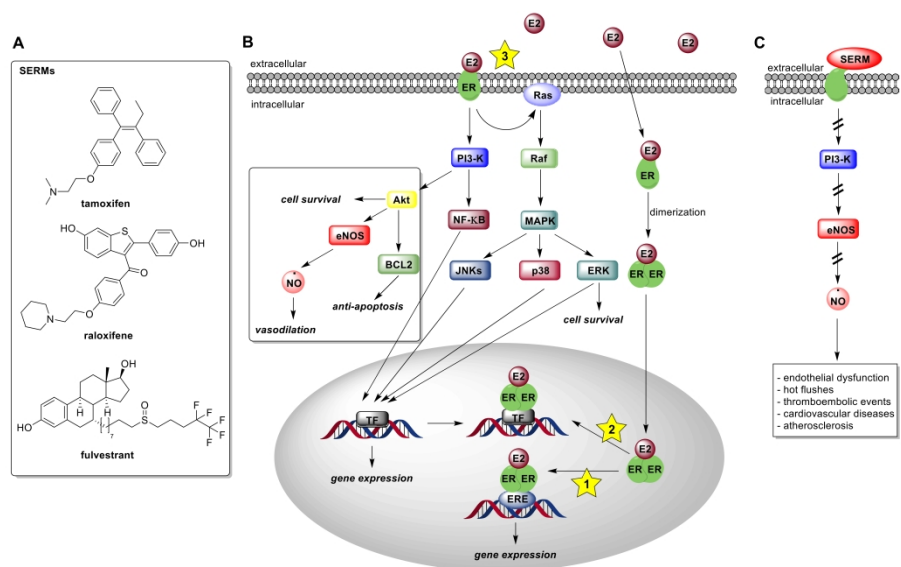
Fig. 1: Structure and modulation of the estrogen signaling by selective estrogen receptor modulators (SERMs). (A) Chemical structure of the SERMs tamoxifen, raloxifene, and fulvestrant. (B) Shown the most important intracellular signaling pathways of 17β-estradiol (E2) that could be influenced by SERMs. Signaling pathway 1 (yellow star): canonical estrogen pathway, the ligand-activated estrogen receptor (ER) binds specifically to the estrogen responsive element (ERE) in the promoter region of the targeted gene. Signaling pathway 2: non-ERE-depending estrogen pathway: the ligand-activated estrogen receptor interacts with other transcription factors (TF), like NF-κB, and, activates gene expression in ERE-independent manner. Signaling pathway 3: non-genomic estrogen pathway, ERs that are localized in cell membrane activate PI3-K/MAPK-signaling and regulate for example vasodilation by an activation of the endothelial nitric oxide (eNOS) synthase (eNOS). Moreover, a ligand-independent mechanism by the activation of different growth factors was described (not shown). (C) In particular, the influence of SERMs on the NO-signaling is coupled with several side effects, like endothelial dysfunction. PI3-K: Phosphatidylinositol-4,5-bisphosphate 3-kinase; Akt: Protein kinase B; MAPK: mitogen-activated protein kinase; NF-κB: Nuclear factor kappa B; BCL2: B-cell lymphoma 2; ERK: extracellular-signal-regulated kinase; JNK: c-Jun N-terminal kinase.
