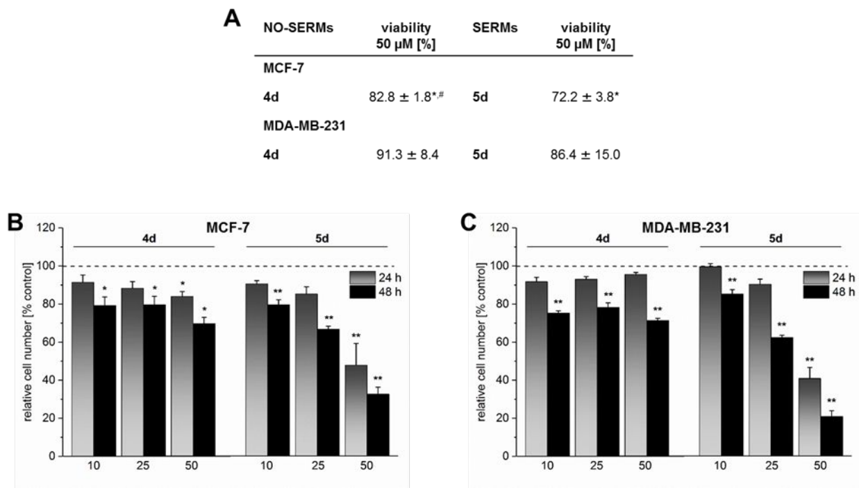
Fig. 6: Influence of NO-SERMs 4 or SERMs 5 on cell viability and proliferation of breast cancer cell lines. (A) Influence of the NO-SERMs 4 and SERMs 5 on cell viability was investigated. Additional release of *NO preserved viability of MCF-7 cells. Three independent experiments were performed (n =9). Mean \pm SEM, ANOVA and Bonferroni post hoc test comparison vs. DMSO control, * p < 0.05 or, ** p < 0.01. Furthermore, the influence of the corresponding compounds 4d and 5d on the number of proliferating cells on (B) MCF-7 and (C) MDA-MB-231 cells was analyzed. In both breast cancer cell lines, the number of proliferating cells was preserved by the additional release of *NO. Four independent experiments were performed (n = 8). Mean \pm SEM, ANOVA and Bonferroni post hoc test comparison vs. DMSO control, * p < 0.05 or, ** p < 0.01.
