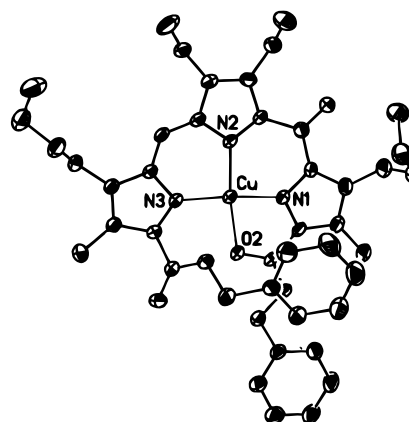
Figure 1. View of complex 2, C_{42}H_{45}N_3O_7Cu \cdot 0.5 CHCl_3 , showing the atom-labeling scheme. Thermal ellipsoids are scaled to the 30% probability level. Hydrogen atoms have been omitted for clarity.
