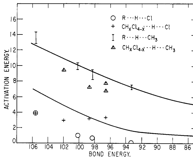
Fig. 7.—Similar to Fig. 6: O, \text{R}\cdots\text{H}\cdots\text{Cl} ; +, \text{CH}_3\text{Cl}_4\text{-X}\cdots\text{H}\cdots\text{Cl} , ref. 13 and J. H. Knox and R. H. Nelson; I, \text{R}\cdots\text{H}\cdots\text{CH}_3 , showing range of reported values; \Delta , \text{CH}_3\text{Cl}_4\text{-X}\cdots\text{H}\cdots\text{CH}_3 , A. F. Trotman-Dickenson, "Gas Kinetics," Academic Press, Inc., New York, N. Y., 1955.
