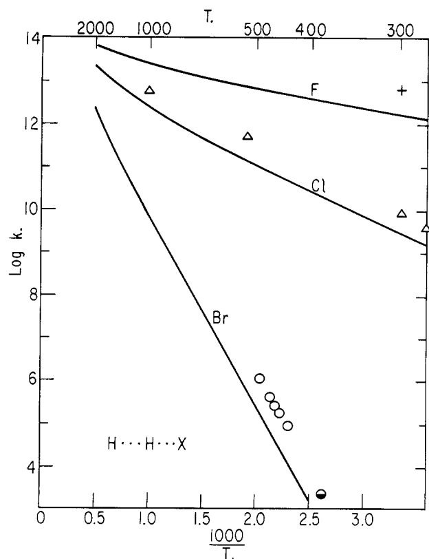
Fig. 8.—Calculated and observed rate constants for halogen atom attack on H_2 : \bullet , Br, and + , F, Fettis, Knox, Trotman-Dickenson, Fig. 6; \circ , Br, M. Bodenstein and H. Lutkemeyer, Z. physik. Chem. , 114 , 208 (1924); \Delta , Cl, H. O. Pritchard, J. B. Pyke, and A. F. Trotman-Dickenson, J. Am. Chem. Soc. , 76 , 1201 (1954).
