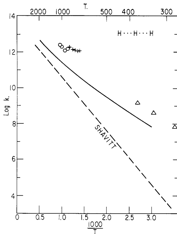
Fig. 1.—Rate constants for para-ortho hydrogen conversion compared with Shavitt's theoretical line, - - -, and a line calculated by this method, —: O, ref. 5; +, ref. 6; \Delta , ref. 7.
