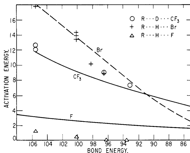
Fig. 6.—Calculated potential energy of activation and observed Arrhenius activation energy plotted against dissociation energy for carbon-hydrogen bonds: O, \text{R}\cdots\text{D}\cdots\text{CF}_3 , ref. 21 and unpublished work by Halbert Carmichael; +, \text{R}\cdots\text{H}\cdots\text{Br} ; \Delta , \text{R}\cdots\text{H}\cdots\text{F} , G. C. Fettis, J. H. Knox, and A. F. Trotman-Dickenson, Can. J. Chem. , 38 , 1643 (1960).
