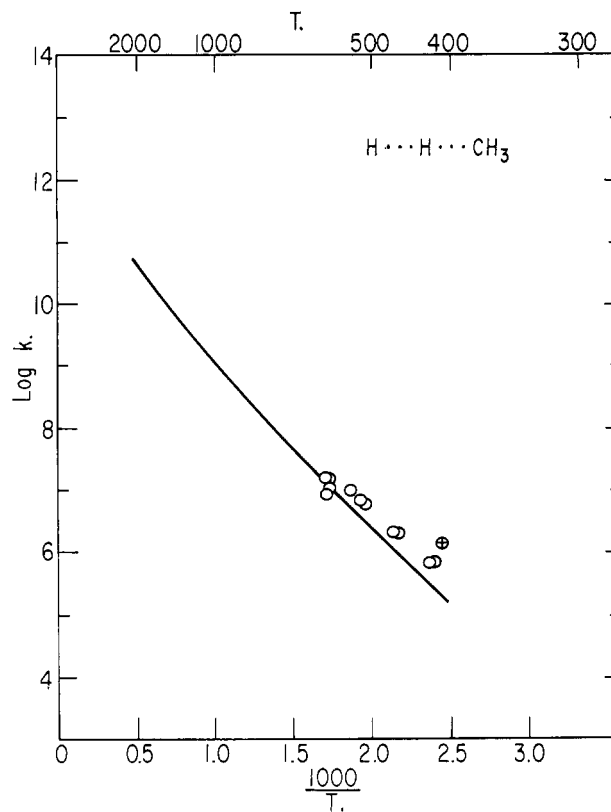
Fig. 9.—Calculated and observed rate constants for methyl radical reaction with H_2 : \circ , T. G. Marjory and E. W. R. Steacie, Can. J. Chem. , 30 , 800 (1952); + , J. C. Polanyi, J. Chem. Phys. , 24 , 493 (1956).
