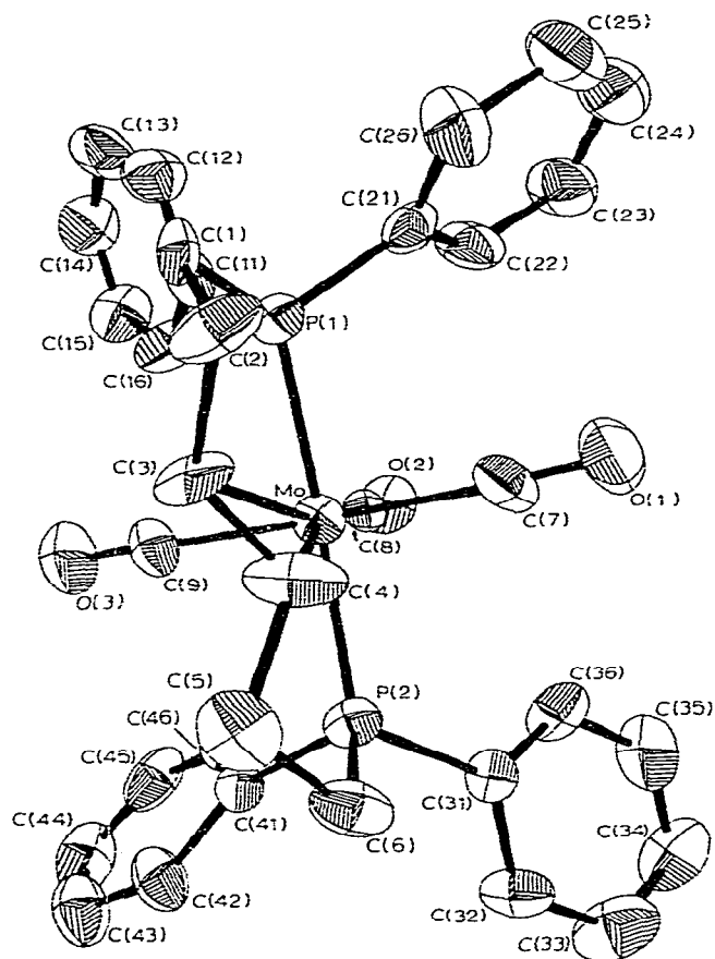
Fig. 1. The molecular geometry, atomic numbering, and anisotropic thermal ellipses (50% probability boundaries) for \text{Mo}(\text{CO})_3(\text{BDPH}) .
