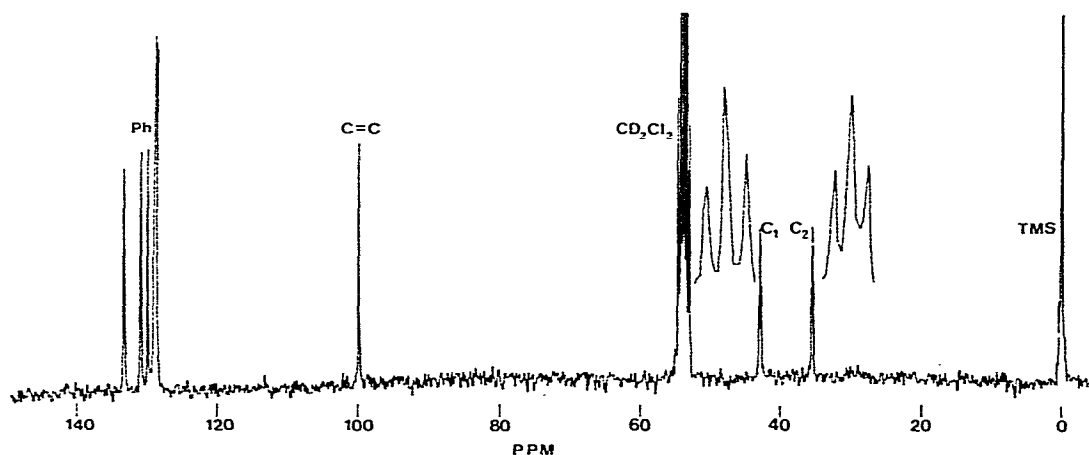
Fig. 4. ^{13}C NMR spectrum of Mo(CO)_3(BDPH) .
