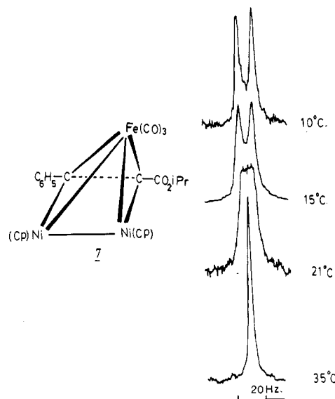
Figure 2. Variable-temperature 80-MHz ^1H NMR spectra of the C_5H_5 protons of 7.
