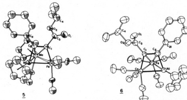
Figure 1. ORTEP diagrams showing structures of molecules 5 and 6 .
