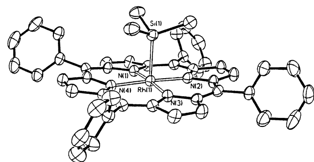
Fig. 2. ORTEP drawing of (5,10,15,20-tetraphenylporphyrinato)(trimethylsilyl)rhodium(III) ( 5 ), (a) and edge view, (b) hydrogens have been omitted for clarity.
