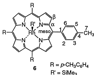
Fig. 1. General structural formula of porphyrin–silyl complexes.
