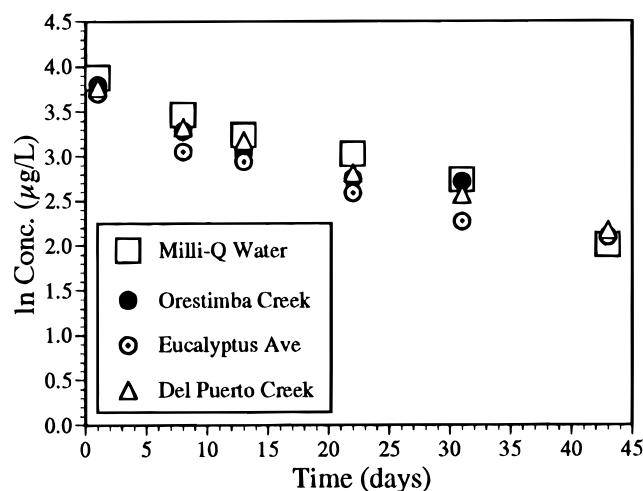
Figure 3. Observed concentration vs time data for diazinon in sterile natural and pH 8.0 phosphate-buffered Milli-Q waters at 40 °C.
