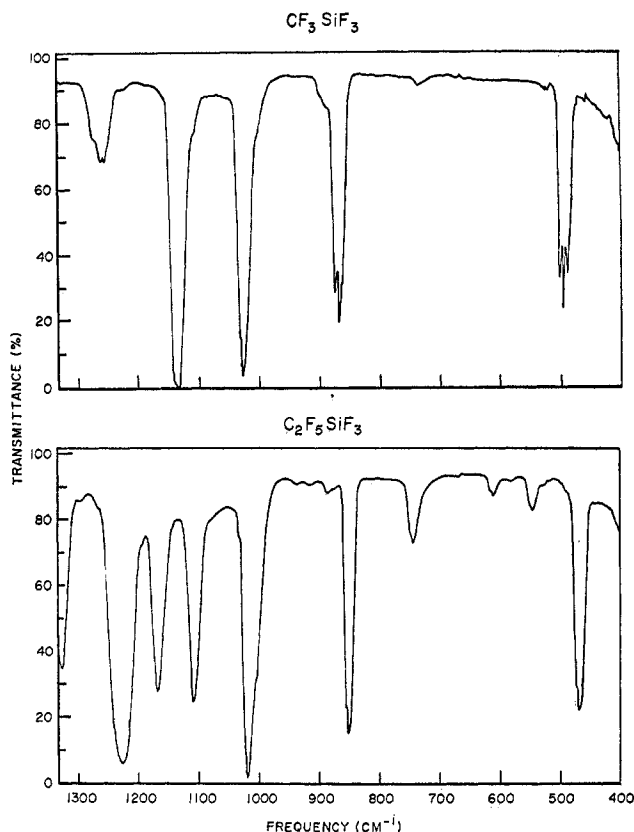
Figure 2.—Infrared spectra of \text{CF}_3\text{SiF}_3 (I) and \text{C}_2\text{F}_5\text{SiF}_3 (II).
