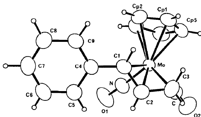
Fig. 1. ORTEP drawing of the endo-cis - [\text{CpMo(NO)(CO)(phenylallyl)}]^+ cation showing 50% probability ellipsoids for non-hydrogen atoms. Hydrogen atoms are shown at refined positions, but with smaller thermal parameters.
