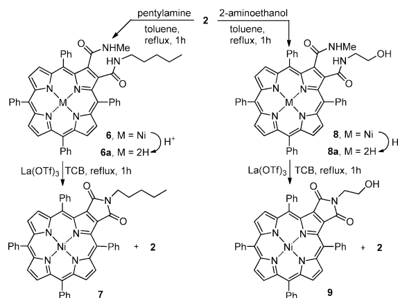
Scheme 3. Synthesis of Porphyrins 6–9 , 6a , and 8a
