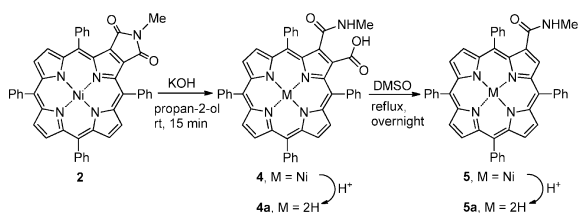
Scheme 2. Synthesis of Porphyrins 4 , 4a , 5 , and 5a
