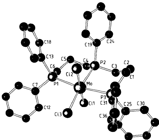
Fig. 2. Molecular arrangement and numbering scheme of the non-hydrogen atoms of 1. Selected bond lengths (pm) and angles (°) are: Cl1–Mo, 243.9(8); Cl2–Mo, 239.6(9); Cl3–Mo, 238.2(8); P1–Mo, 259.8(8); P2–Mo, 253.0(9); P3–Mo, 255.5(8). Cl2–Mo–Cl1, 177.0(3); Cl3–Mo–Cl1, 90.4(3); Cl3–Mo–Cl2, 92.5(3); P1–Mo–Cl1, 86.7(3); P1–Mo–Cl2, 93.8(3); P1–Mo–Cl3, 98.8(3); P2–Mo–Cl1, 82.1(3); P2–Mo–Cl2, 94.9(3); P2–Mo–Cl3, 171.1(3); P2–Mo–P1, 85.7(3); P3–Mo–Cl1, 96.5(3); P3–Mo–Cl2, 82.6(3); P3–Mo–Cl3, 90.4(3); P3–Mo–P1, 170.2(3); P3–Mo–P2, 85.6(3).
