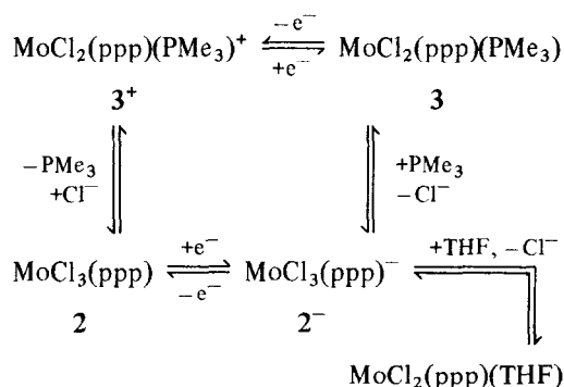
Scheme 1. Electrochemical and chemical reactions of 2 occurring in THF in the absence and presence of \text{PMe}_3 ; \text{ppp} = \text{MeP}(\text{CH}_2\text{CH}_2\text{CH}_2\text{PMe}_2)_2 .
