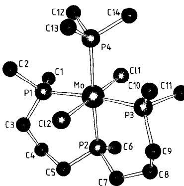
Fig. 4. Molecular structure of 3. Important interatomic distances (pm) and angles (°) are: Cl1–Mo, 245.5(6); Cl2–Mo, 243.4(7); P1–Mo, 252.1(8); P2–Mo, 246.8(7); P3–Mo, 247.7(8); P4–Mo, 251.2(8). Cl2–Mo–Cl1, 179.3(3); P1–Mo–Cl1, 93.7(3); P1–Mo–Cl2, 86.4(2); P2–Mo–Cl1, 91.5(2); P2–Mo–Cl2, 89.1(2); P2–Mo–P1, 88.4(3); P3–Mo–Cl1, 93.4(3); P3–Mo–Cl2, 86.5(3); P3–Mo–P1, 172.4(3); P3–Mo–P2, 88.9(3); P4–Mo–Cl1, 84.4(2); P4–Mo–Cl2, 95.0(3); P4–Mo–P1, 92.0(3); P4–Mo–P2, 175.9(3); P4–Mo–P3, 91.2(3).
