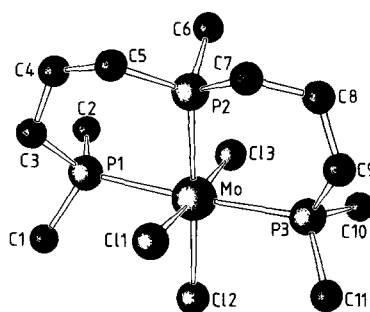
Fig. 3. The structure of 2. Important interatomic distances (pm) and angles (°) are: Cl1–Mo, 241.9(3); Cl2–Mo, 244.3(3); Cl3–Mo, 239.6(3); P1–Mo, 254.5(3); P2–Mo, 249.8(3); P3–Mo, 253.1(4). Cl2–Mo–Cl1, 91.7(1); Cl3–Mo–Cl1, 175.8(1); Cl3–Mo–Cl2, 92.5(1); P1–Mo–Cl1, 89.2(1); P1–Mo–Cl2, 94.5(1); P1–Mo–Cl3, 90.8(1); P2–Mo–Cl1, 83.6(1); P2–Mo–Cl2, 175.3(1); P2–Mo–Cl3, 92.2(1); P2–Mo–P1, 84.7(1); P3–Mo–Cl1, 88.8(1); P3–Mo–Cl2, 90.2(1); P3–Mo–Cl3, 90.8(1); P3–Mo–P1, 175.0(1); P3–Mo–P2, 90.5(1).
