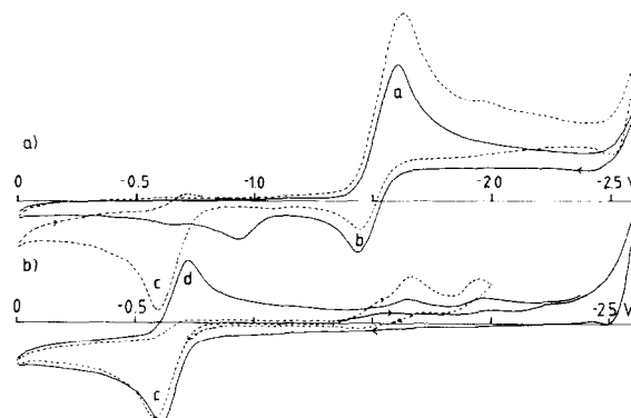
Fig. 1. (a) Cyclic voltammograms of 2 (100 mV/s); —: pure complex; ---: with added \text{PMe}_3 . (b) Cyclic voltammograms of 3 (100 mV/s); —: pure complex; ---: in the presence of \text{Et}_4\text{NCl} .
