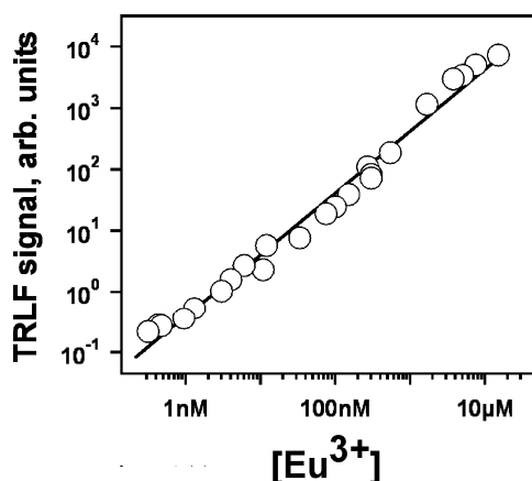
Figure 2. The concentration plot for TRLF signal for a magnetic microsphere assay using AMS-40-5a microspheres. Linearity of TRLF detection for magnetic extraction of \text{Eu}^{3+} by AMS-40 microspheres modified by 5a in the presence of TTA.
