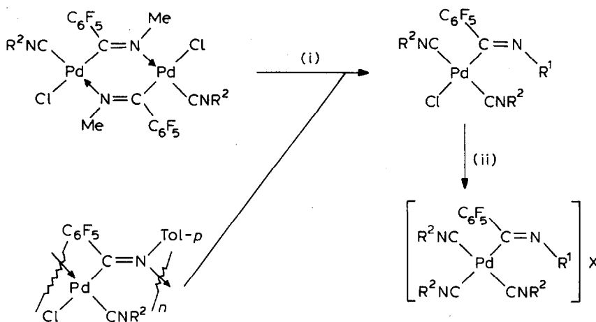
SCHEME 1. (i) + \text{CNR}^2 , \text{CH}_2\text{Cl}_2 ; (ii) + \text{CNR}^2 + \text{NaX} ( \text{X} = \text{ClO}_4 in acetone or \text{BPh}_4 in \text{CH}_2\text{Cl}_2 ).
