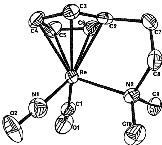
Fig. 1. ORTEP drawing of [\eta^5\text{-}\eta^1\text{-C}_5\text{H}_4\text{CH}_2\text{CH}_2\text{N}(\text{CH}_3)_2\text{Re}(\text{NO})(\text{CO})]^+ \text{BPh}_4^- ( 5b ). The \text{BPh}_4^- anion is omitted for simplicity.
