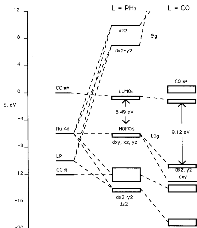
Fig. 1. Molecular orbital diagram for [\text{RuL}_4(-\text{C}\equiv\text{C}-p-\text{C}_6\text{H}_4-\text{C}\equiv\text{C}-\text{H})_2] ( \text{L} = \text{PH}_3 (10); \text{CO} (17)).
