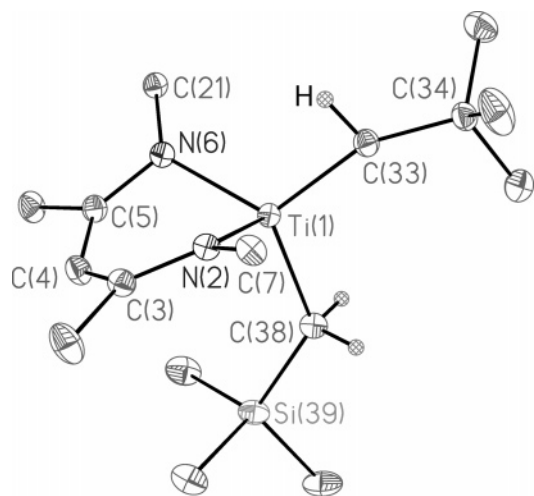
Figure 1. Perspective view of 1 with thermal ellipsoids at the 50% probability level. Hydrogens, with the exception of \alpha -hydrogens, and aryl groups on the \beta -diketiminate, with the exception of ipso carbons C(7) and C(21), have been omitted for clarity. The \alpha -hydrogens on C(33) and C(38) were located and refined isotropically. Table 1 lists pertinent metrical parameters.
