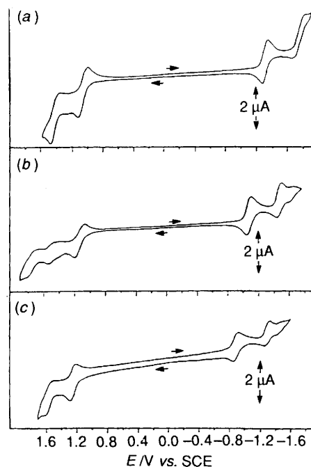
Fig. 4 Cyclic voltammograms of \text{In}(\text{por})[\text{N}_4\text{C}(\text{CMe}_3)] for por = oep (a), tpp (b) or tfpp (c), in \text{CH}_2\text{Cl}_2 , 0.1 \text{ mol dm}^{-3} \text{NBu}_4\text{ClO}_4 . Scan rate = 100 \text{ mV s}^{-1}
