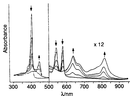
Fig. 8 Time-resolved UV/VIS spectra taken during the first reduction of \text{In}(\text{oep})[\text{N}_4\text{C}(\text{CMe}_3)] in \text{CH}_2\text{Cl}_2 , 0.1 \text{ mol dm}^{-3} \text{NBu}_4\text{ClO}_4
