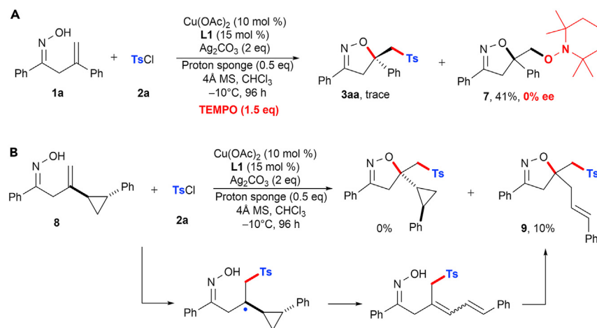
Scheme 3. Mechanistic Study
