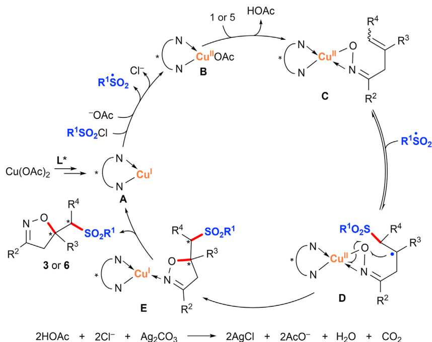
Figure 5. Mechanistic Proposal
