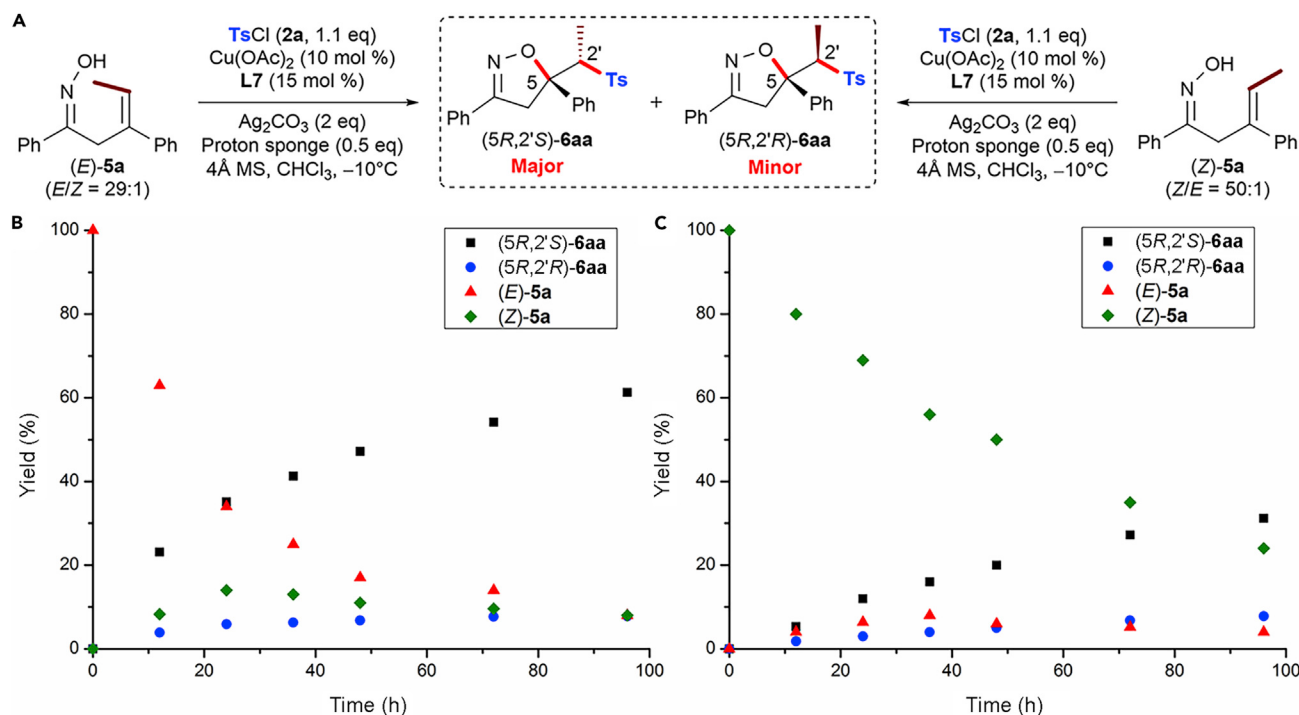
Figure 2. Time-Course Experiments
