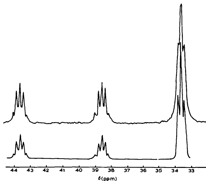
Fig. 1. Observed and calculated ^{31}\text{P}\{^1\text{H}\} NMR spectra of trans - [\text{RhCl}(\text{CO})(\text{cis-Mo}(\text{CO})_4(\text{TPM}))_2] in \text{C}_6\text{D}_6 at 28^\circ\text{C} .
