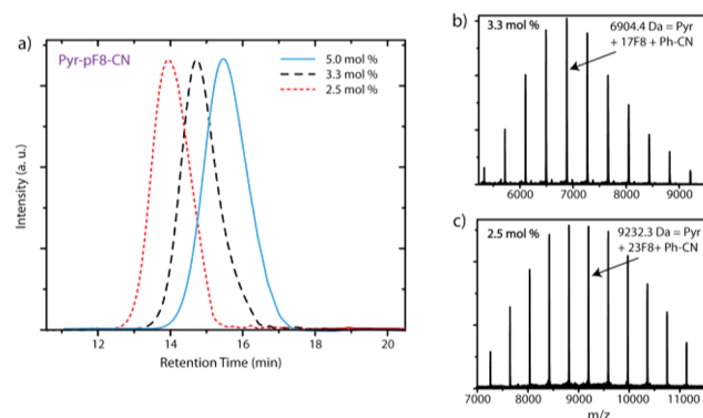
Figure 6. (a) GPC profiles of 1 with Pyr-Pd-( t Bu 3 P)Br obtained at initiator ratio of 5.0 mol % (solid blue), 3.3 mol % (dashed black), and 2.5 mol % (dotted red). The unimodal curves show a shift to lower retention time (which corresponds to higher M_n ) when a lower feed ratio between the monomer and the initiator was used, while preserving low PDI (1.21–1.25). The GPC chromatograms were obtained after removing the monomer from the mixture (by precipitation with methanol). MALDI-TOF mass spectra of (b) 3.3 and (c) 2.5 mol %. For MALDI-TOF spectrum of 5.0 mol % please see Figure S7.
