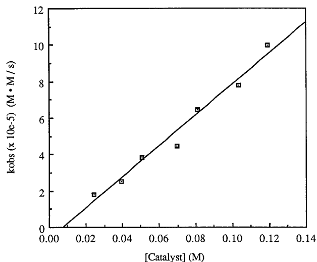
Figure 6. A plot of k_{\text{obs}} versus catalyst concentration for polymerizations of n -hexyl isocyanate using 2.
