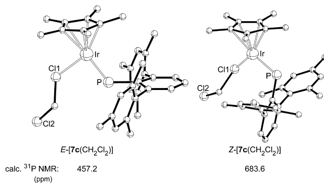
Figure 3. Intermediate E - and Z -[ 7c ( \text{CH}_2\text{Cl}_2 )] calculated at the BP86/TZP level of theory. Hydrogen atoms are omitted for clarity. Selected bond lengths [Å] and angles [deg] for E -[ 7c ( \text{CH}_2\text{Cl}_2 )] and Z -[ 7c ( \text{CH}_2\text{Cl}_2 )] (in square brackets): Ir–P 2.192 [2.206], Ir–C11 2.567 [2.368]; Ir–P–Dmp 125.2 [114.6], P–Ir–C11 87.5 [102.9].
