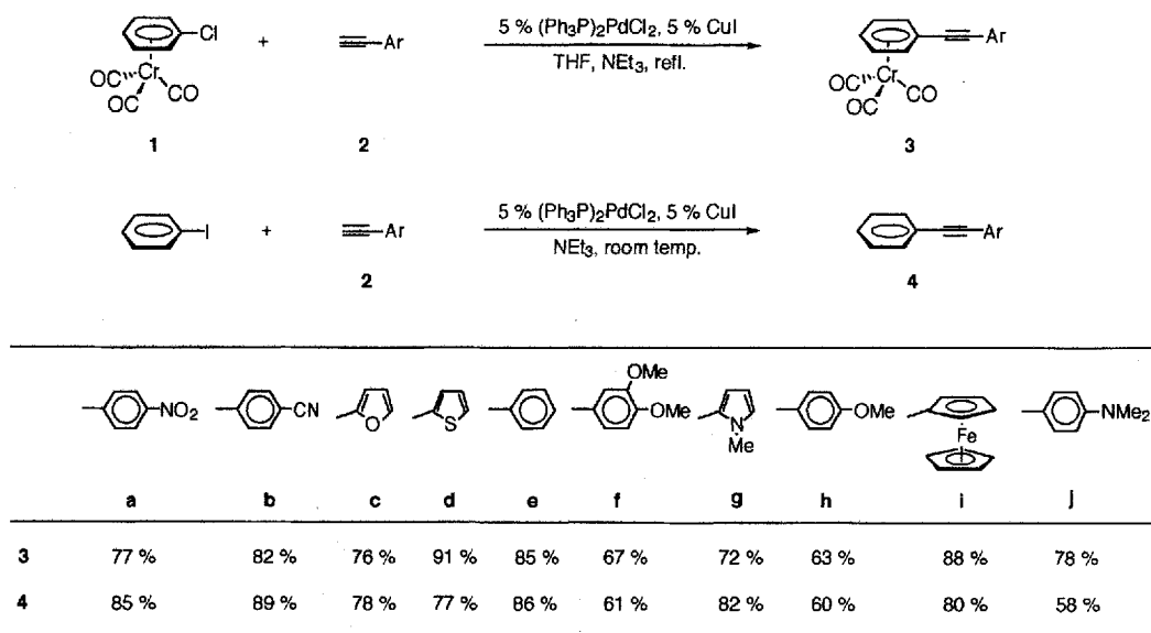
Scheme 2. Syntheses of the complexes 3 and the free ligands 4
