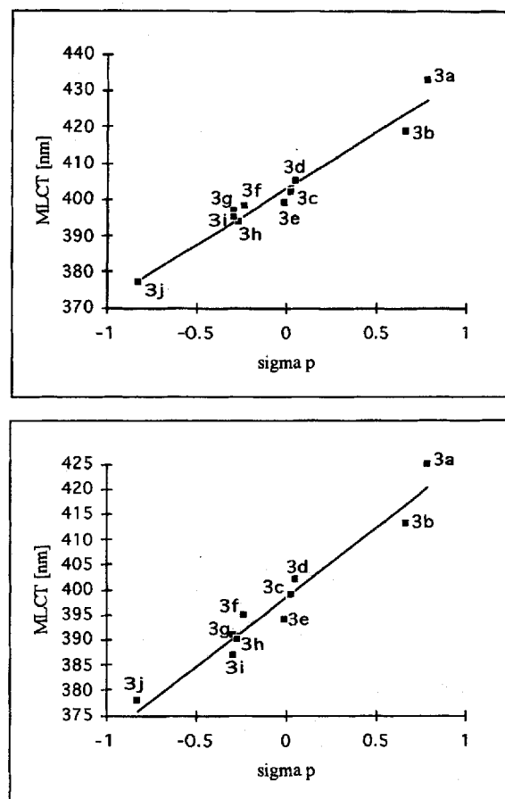
Figure 3. (top) \lambda_{\text{max}}(\text{MLCT, CH}_2\text{Cl}_2) - \sigma_p plot ( r = 0.978 ; s = 1.057 nm) and (bottom) \lambda_{\text{max}}(\text{MLCT, CH}_3\text{CN}) - \sigma_p plot ( r = 0.972 ; s = 1.056 nm); (top) regression line \lambda_{\text{max}}(\text{MLCT, CH}_2\text{Cl}_2) = 403 + 31.1 \sigma_p [nm]; (bottom) regression line \lambda_{\text{max}}(\text{MLCT, CH}_3\text{CN}) = 399 + 27.6 \sigma_p [nm]
