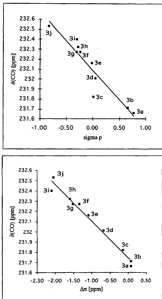
Figure 2. (top) \delta(\text{CO}) - \sigma_p plot ( r = 0.936 ; s = 0.036 ppm) and (bottom) \delta(\text{CO}) - \Delta_\pi plot ( r = 0.987 ; s = 0.026 ppm); (top) regression line \delta(\text{CO}) = 232.09 - 0.59 \sigma_p [ppm]; (bottom) regression line \delta(\text{CO}) = 231.75 - 0.36 \Delta_\pi [ppm]
