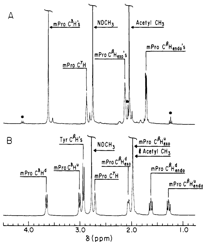
Figure 2. ^1\text{H} NMR spectra of (A) Ac-2,4-MePro-NHMe and (B) Ac-L-Tyr-2,4-MePro-NHMe in \text{D}_2\text{O} solution at 25 °C. In order to determine if the unlabeled minor resonances present in the A spectrum are due to a contaminating molecule, the peptide was recrystallized several times from ethyl acetate. The material used to obtain this spectrum (A) comes from a dissolved single crystal. Peaks marked with an asterisk correspond to small amounts of ethyl acetate associated with this crystal.
