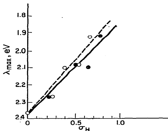
Fig. 5. \lambda_{\max} of p -substituted 4-phenylazo-1-naphthol vs. Hammett \sigma value of p -substituent; • — \sigma_H ; ○ — \sigma_{uv,K} .
