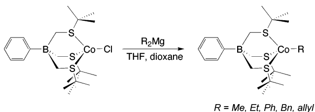
Scheme 1. Synthesis of [\text{PhTt}^{\text{tBu}}]\text{Co}(\text{R}) Complexes
