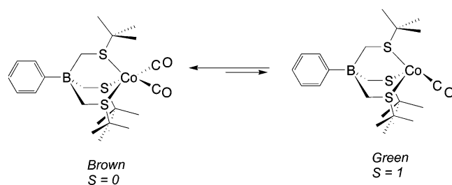
Scheme 4. Equilibrium between [\text{PhTt}^{\text{tBu}}]\text{Co}(\text{CO})_2 and [\text{PhTt}^{\text{tBu}}]\text{Co}(\text{CO})
