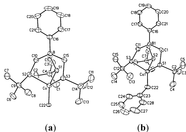
Figure 1. Thermal ellipsoid plots of (a) [\text{PhTt}^{\text{tBu}}]\text{Co}(\text{Me}) and (b) [\text{PhTt}^{\text{tBu}}]\text{Co}(\text{Bn}) . Thermal ellipsoids are drawn at 30% probability. Hydrogen atoms have been omitted for clarity.
