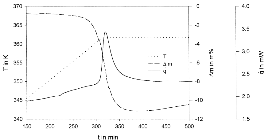
Fig. 5. TG/DSC curves of \text{BH}_3\text{NH}_3 at isothermal temperature 363 K: (—) heat flow, (●●●) temperature, (— —) mass loss.
