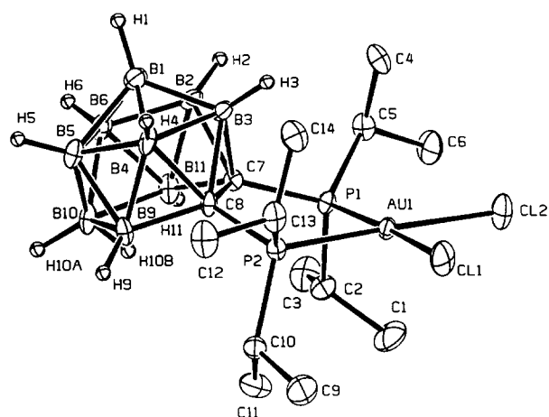
Fig. 2. Simplified ORTEP plot of [\text{AuCl}_2(\text{nip})] . Thermal ellipsoids are shown at 30% probability levels, except for H atoms which are drawn with an isotropic displacement parameter of 1.0.
