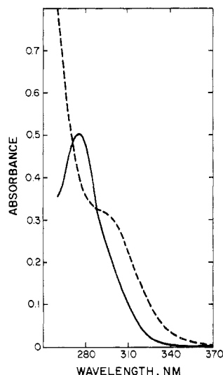
Figure 2. Spectral change accompanying the conversion of Cu[HB(pz) 3 ](CO) to Cu[HB(pz) 3 ](NBD) in a two-component spectrophotometer cell: —, spectrum observed when hexane solutions of Cu[HB(pz) 3 ](CO) and NBD occupy separate compartments; ----, spectrum resulting when the two solutions are mixed.
