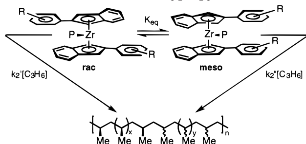
Scheme 1. Proposed Mechanism for Formation of Elastomeric Polypropylene
