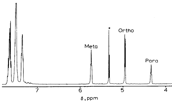
Fig. 1. Low-field region of the 400 MHz ^1\text{H} NMR spectrum of [\text{RuCl}(\text{dppb})(\eta^6\text{-toluene})]^+ \text{PF}_6^- in \text{CD}_2\text{Cl}_2 ; \star represents \text{CHDCl}_2/\text{CH}_2\text{Cl}_2 impurities in the solvent.
