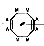
C_{2v} symmetry
