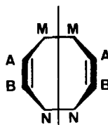
C_s symmetry
