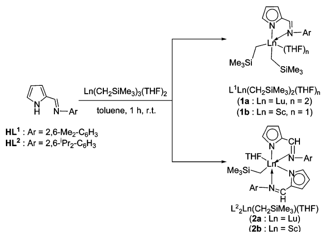
Scheme 1. Synthetic Pathway for Preparation of Complexes 1a , 1b , 2a , and 2b
