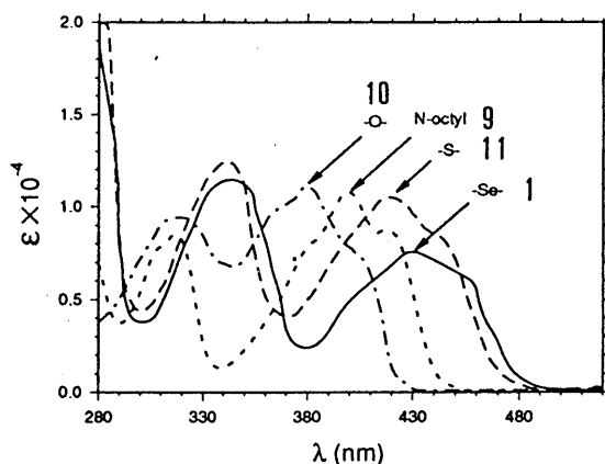
Fig. 1. Ultraviolet Spectra of 5-Deazaflavin Related Compounds in Acetonitrile
