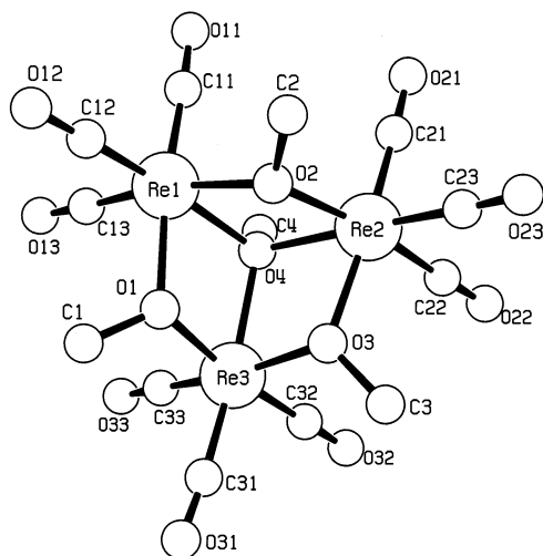
Fig. 2. Structure of the anion of [\text{Pt}_2\text{Re}(\mu_3\text{-S})_2(\text{PPh}_3)_4(\text{CO})_3][\text{Re}_3(\mu_3\text{-OMe})_3(\mu_3\text{-OMe})(\text{CO})_9] ( 3a ).
