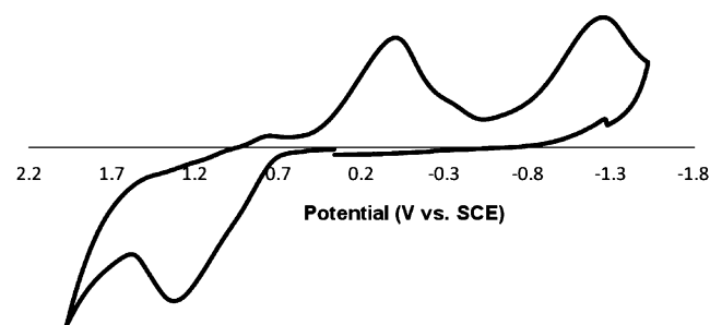
Figure 4. Cyclic voltammogram of complex 1 vs SCE. Potential sweep from +0.38 V to +2.0 V to -1.5 \text{ V} and back to +0.38 V.
