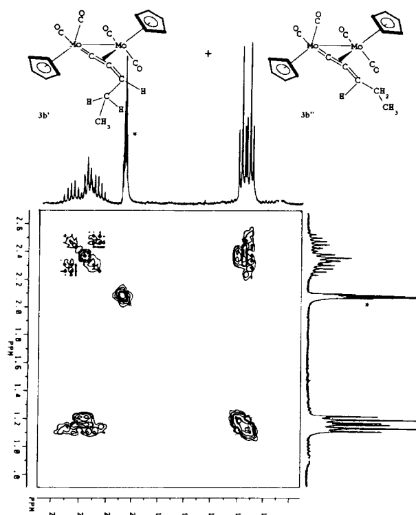
Fig. 3. 2D ^1H NMR spectrum of 3b .
