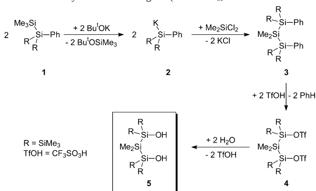
Scheme 1. Synthesis of the Ligand ( R = \text{SiMe}_3 )
