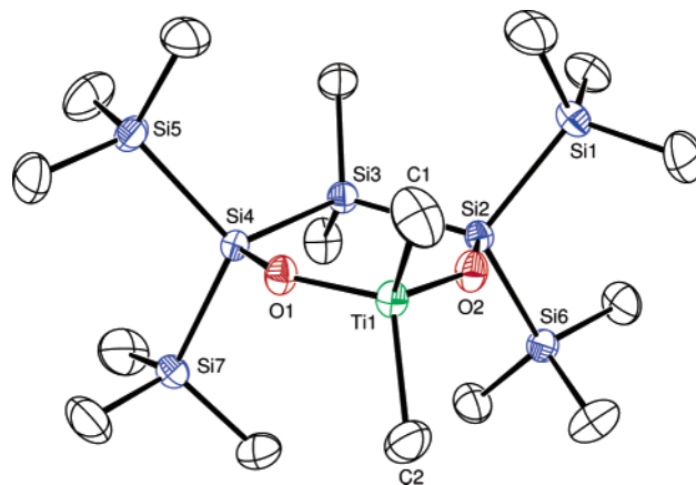
Figure 4. Molecular structure of 10 in the crystal. The thermal ellipsoids correspond to 50% probability. Hydrogen atoms are omitted for clarity. Selected bond lengths [Å] and angles [deg]: \text{Ti1}-\text{C2} 2.0787(18), \text{Ti1}-\text{C1} 2.0829(19), \text{O2}-\text{Ti1}-\text{O1} 108.19(5), \text{O2}-\text{Ti1}-\text{C2} 107.82(7), \text{O1}-\text{Ti1}-\text{C2} 111.24(7), \text{O2}-\text{Ti1}-\text{C1} 110.62(7), \text{O1}-\text{Ti1}-\text{C1} 109.94(7), \text{C2}-\text{Ti1}-\text{C1} 109.01(9).
