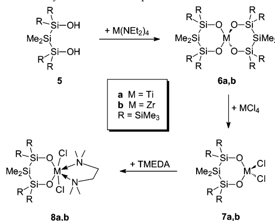
Scheme 2. Syntheses of the Complexes 6–8
