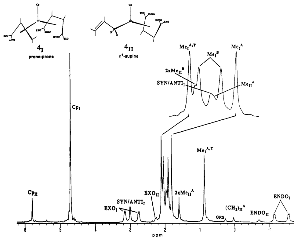
Figure 4. Isomers of \text{Cp}(1,1,2\text{-Me}_3\text{allyl})(2,3\text{-Me}_2\text{butadiene})\text{Hf} ( 4 ) along with ^1\text{H} NMR spectrum measured in toluene- d_8 at -94^\circ\text{C} . Peak positions and coupling constants are given in the Experimental Section. Subscripts I and II refer to isomers 4 I and 4 II . Superscripts A and B refer to the allyl and butadiene ligands, respectively. Superscript T refers to the terminal allyl positions (these two peaks coalesce at +95^\circ\text{C} ). In the absence of these superscripts: SYN/ANTI I refers to the allyl protons in 4 I ; EXO and ENDO refer to the butadiene \text{CH}_2 protons. GRS is silicone stopcock grease, used as a reference ( \delta 0.26). The peaks labeled SYN/ANTI I are COSY correlated.
