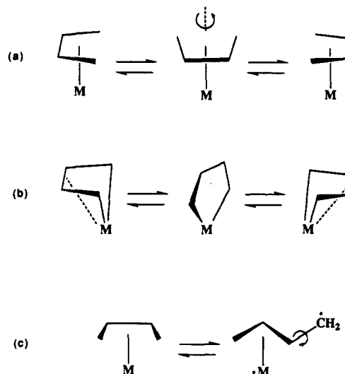
Figure 3. Fluxional processes for metal-diene complexes: (a) diene rotation about the metal-to-diene centroid axis; (b) envelope-flip mechanism; (c) slip mechanism. Only the latter two mechanisms can effect endo-exo exchange.
