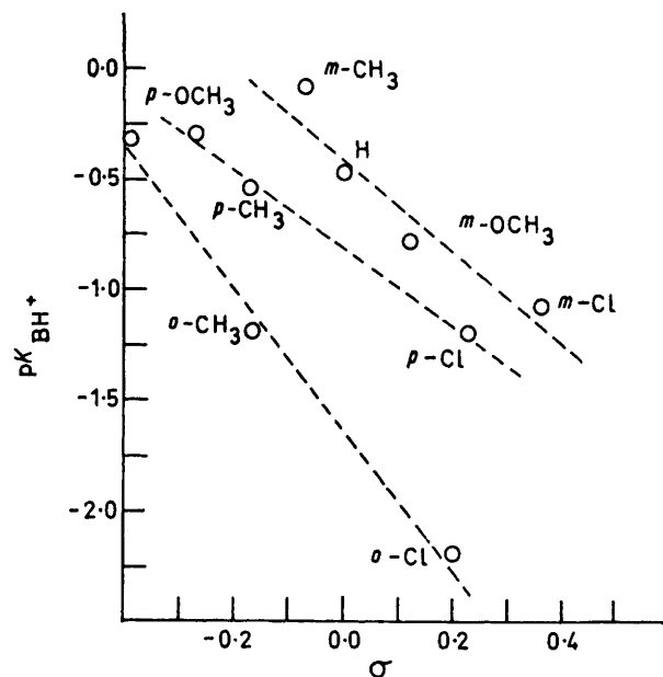
FIGURE 3 Dependence of pK_{BH^+} values of 1-arylaazo-4-methoxynaphthalenes on Hammett \sigma values
