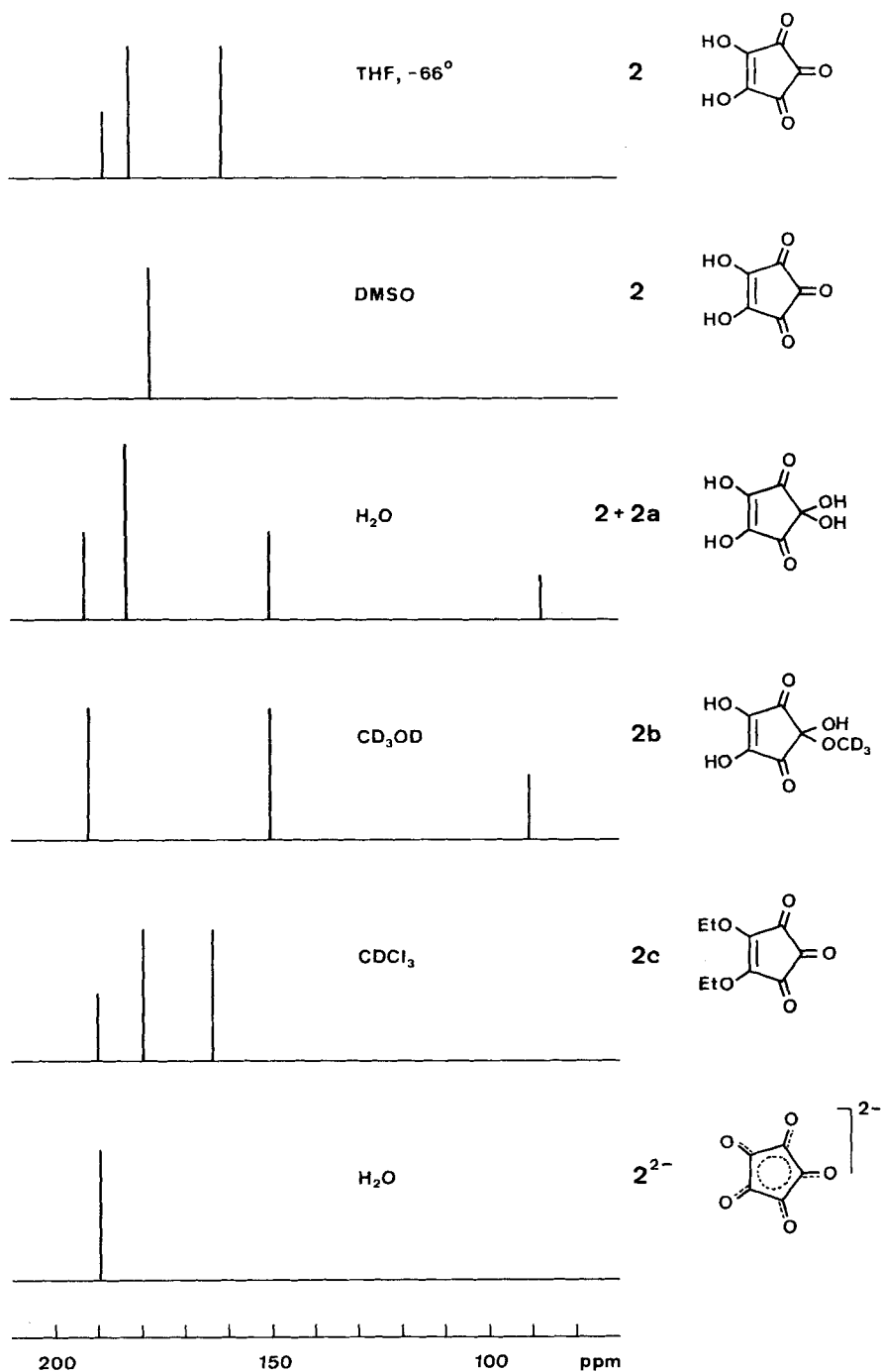
Fig. 2. ^{13}\text{C} -NMR. spectra of croconic acid ( 2 ) and derivatives (idealized peak heights). T = 30^{\circ} , top spectrum at -66^{\circ}
