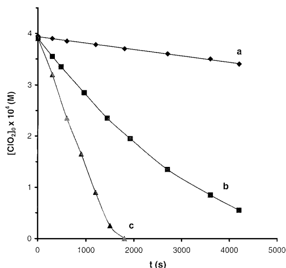
Figure 1. \text{ClO}_2 concentration as a function of time under illumination with 460 nm light. P = 1.46 \text{ mW dm}^{-3} , T = 25^\circ\text{C} , and [\text{I}_2]_0 = 0.0 (a), 1.45 \times 10^{-4} (b), and 5.08 \times 10^{-4} \text{ M} (c).
