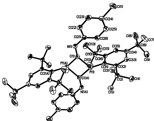
Fig. 3. Molecular structure of \text{Mes}^*\text{P}(\mu\text{-CNPh})_2\text{PMes}^* . Selected bond lengths ( \text{\AA} ) and angles ( ^{\circ} ): \text{P}(1)\text{--C}(1) 1.829(2), \text{P}(1)\text{--C}(1\text{A}) 1.813(2), \text{P}(1)\text{--C}(31) 1.845(2), \text{P}(1)\text{--P}(1\text{A}) 2.674(1), \text{Cl}(1)\text{--C}(24) 1.741(3), \text{N}(1)\text{--C}(1) 1.282(3), \text{N}(1)\text{--C}(21) 1.405(3), \text{C}(1)\text{--P}\text{--C}(1\text{A}) 85.5(1), \text{C}(1)\text{--P}\text{--C}(31) 122.2(1), \text{C}(1\text{A})\text{--P}\text{--C}(31) 121.9(1), \text{C}(1)\text{--N}(1)\text{--C}(21) 124.8(2), \text{N}(1)\text{--C}(1)\text{--P}(1) 139.3(2), \text{N}(1)\text{--C}(1)\text{--P}(1\text{A}) 125.8(2), \text{P}(1)\text{--C}(1)\text{--P}(1\text{A}) 94.5(1).
