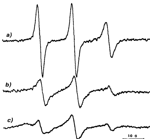
Fig. 7. EPR spectra of 7 (22 mmol) a) before and b)c) after annealing with an equivalent amount of (\text{dA})_{15} or (\text{dA})_n , respectively. In 100 mM NaCl/10 mM \text{MgCl}_2 /10 mM Na-cacodylate (pH 7) buffer at 20°.
