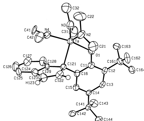
Figure 4. Molecular structure of [Ta(OC 6 H 2 { \eta^1 -Ind}-2-Bu t 2 -4,6)(NMe 2 ) 3 ] ( 8 ).
