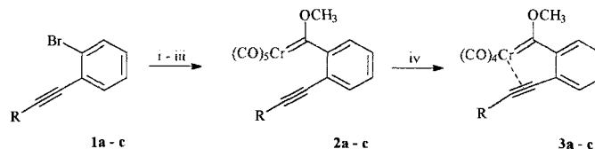
Scheme 2. Synthesis of 2a–c and 3a–c . R = Ph ( 1a , 2a , 3a ), n Pr ( 1b , 2b , 3b ), Si(CH 3 ) 3 ( 1c , 2c , 3c ). Reagents and conditions: i) n -BuLi, Et 2 O, 0 °C; ii) [Cr(CO) 6 ], 0 °C → room temperature; iii) (CH 3 ) 3 OBf 4 , CH 2 Cl 2 ; iv) hv, Et 2 O, –40 °C.
