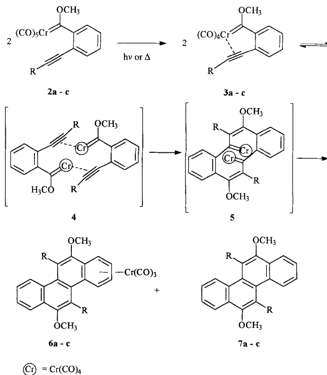
Scheme 5. Suggested mechanism for chrysene formation.
