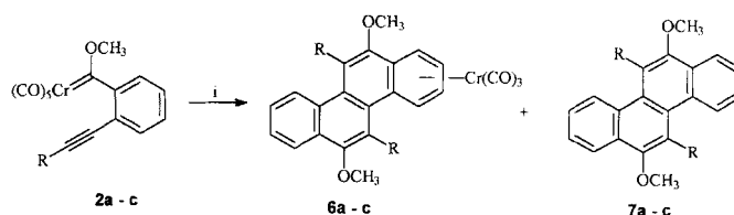
Scheme 3. Synthesis of chrysenes 6a–c and 7a–c . R = Ph ( 2a , 6a , 7a ), n Pr ( 2b , 6b , 7b ), Si(CH 3 ) 3 ( 2c , 6c , 7c ). Conditions: i) t BuOCH 3 , 55 °C.
