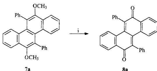
Scheme 4. Oxidation of 7a to 8a . Reagents and conditions: i) (\text{CH}_3)_3\text{SiI} , \text{CH}_2\text{Cl}_2 , room temperature, air, 79 h.
