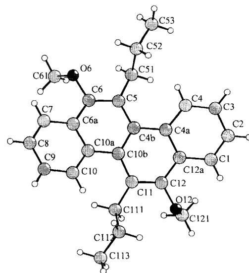
Figure 4. Structure of 7b .
